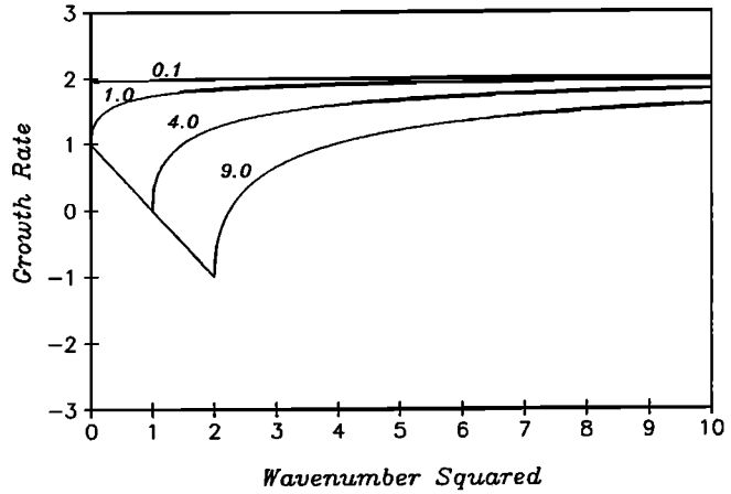
Fig. 10. Plot of the growth rate Re(\sigma_1) from (27) as a function of k^2 . Here Re(\sigma_1) is divided by 1/2 df/dw|_{w_0} and k^2 is divided by \frac{7}{6} df/dw|_{w_0} . Four values of the parameter \gamma/4 df/dw|_{w_0} are illustrated. All curves asymptote to 2 for large wavenumbers.
