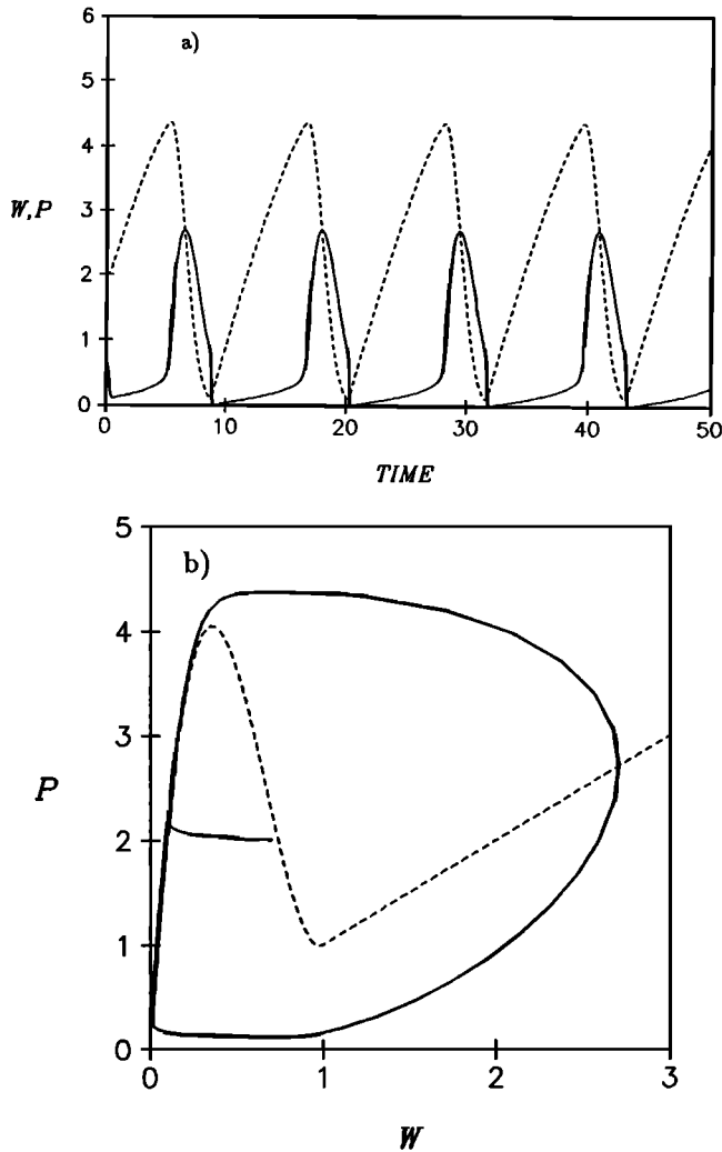
Fig. 7 (a) Numerical solution of (16) with \partial/\partial y = 0 and (17) for p (dashed curve) and w (solid curve) with (A, Q, \gamma) = (50.0, 0.7, 1.0) . (b) p-w phase plane plot of the solution (solid curve). The steady state relation p_0 = f(w) from (18) is also shown (dashed curve).
