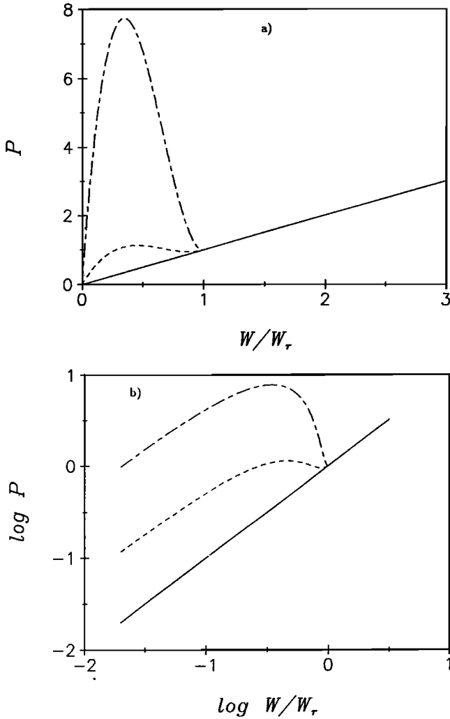
Fig. 6. (a) Pressure drop across the slot calculated from equation (11) as a function of velocity of the fluid for the three values A = 0 (solid curve), 10 (dashed curve), and 100 (dash-dot curve). (b) The same data plotted as log-log.
