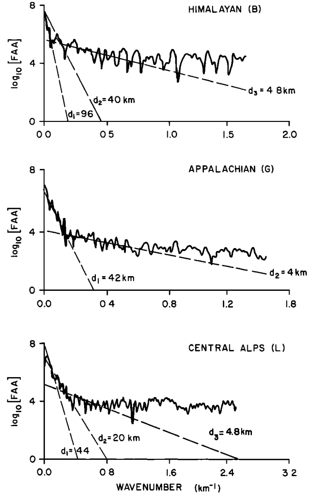
Fig. 13. Plot of wave number versus the logarithm of the free air gravity anomaly power for representative profiles of the Himalaya, Appalachian, and Alpine mountains. Linear segments of the power spectra suggest the existence of discrete density boundaries, the slope being an estimate of their mean depth. Superimposed solid lines on the power spectra represent a least squares fit to the observed linear segments. The gravity energy of these mountains appear to be associated with three main interfaces, d_1 , the M discontinuity; d_2 , an intra-crustal layer; and d_3 , the basement underlying the flexural basin.
