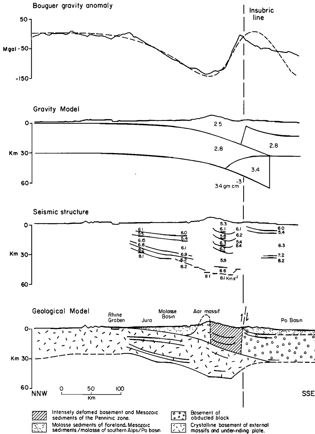
Fig. 16. Bouguer gravity anomaly, seismic structure, and gravity and geological models along the Swiss geotraverse [Rybach et al., 1980]. The gravity model is based on the flexural scheme presented in this paper. In particular, three loads have been considered in deriving the deformation of the basement: the obducted crustal block ( \rho = 2.8 \text{ g cm}^3 ), a subcrustal load ( \rho = 3.4 ), surface topographic load ( \rho = 2.7 ), and sediment infill ( \rho = 2.5 ). The geological model is a schematic cross section based on the gravity model and is generally consistent with previous regional geological interpretations [e.g., Trümpy, 1973].
