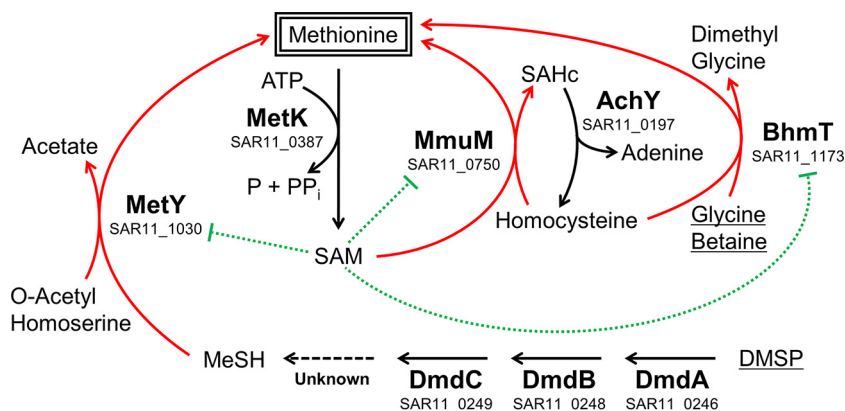
FIG 1 Products of genes with increased expression as DMS becomes limiting. MetY, BhmT, and MmuM work independently to produce methionine, a key organic sulfur compound. Glycine betaine and DMS are underlined to indicate their availability in the growth medium. Red lines indicate increased mRNA and/or protein expression in sulfur-limited exponential-phase samples ( n = 3 ) relative to the expression in control exponential-phase samples ( n = 4 ). Green lines denote the model for inhibition of translation by SAM-sensing riboswitches. DMS, dimethylsulfoniopropionate; MeSH, methanethiol; SAHc, S-adenosyl homocysteine; SAM, S-adenosyl methionine.
