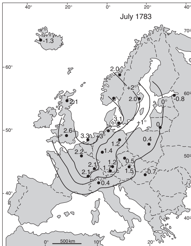
Figure 8. Deviation of the 1783 July surface temperatures from the 1768–1798 mean. Numbers are given in degrees centigrade and the distribution of the anomaly is indicated by isotherms, drawn at 1°C intervals.
