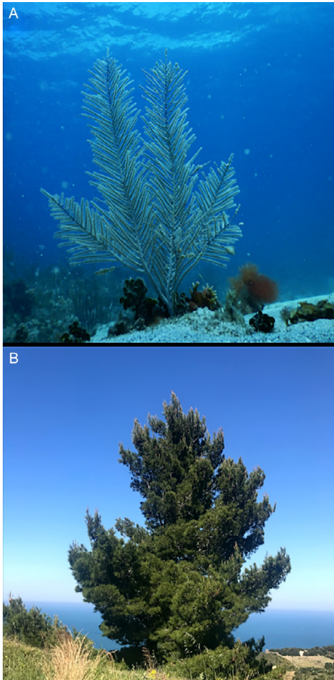
Fig. 11 Branching morphology. (A) Muriceopsis sp. (B) Pinus sp.
