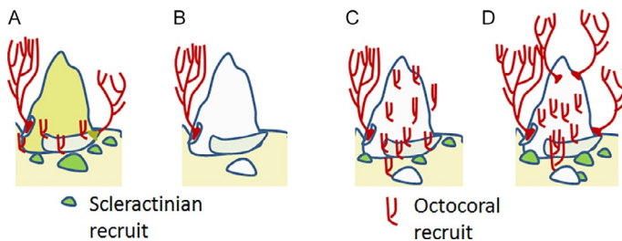
Fig. 5 Schematic illustrating hypotheses by which octocorals attain enhanced resilience following disturbance, and promoting an octocoral-dominated community ((A–D) in a chronology). (A) A coral reef before a major disturbance with a few large colonies of scleractinians and octocorals, as well as their recruits. Differences in recruit positioning reflect dissimilar settlement niches, and octocorals are constrained by their inability to settle on living scleractinians. (B) Immediately after a disturbance that has killed many scleractinians and some octocorals. (C) Octocorals and scleractinians recruit. The altered abundance and distribution of octocorals relative to scleractinians reflects differences in larval supply, and the increase in substrata matching octocoral settlement niches. (D) With time, mature octocorals dominate the benthos. Canopy effects on recruitment enhance self-seeding, which differentially benefits octocorals due to their greater abundance and high reproductive output. Macroalgae, which are not shown, are common in (B–D) and have less effect on octocorals due to the octocorals' escape in size (height).
