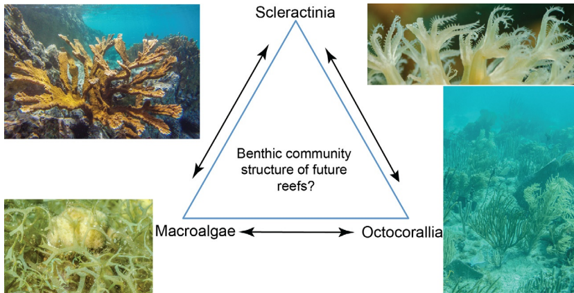
Fig. 2 Schematic illustrating the community structure of present-day reefs in the tropical western Atlantic in which scleractinians, macroalgae, and octocorals compete for dominance. Sponges can also occupy substantial portions of benthic space, but time series data for this taxon are sparse, and in St. John, they do not appear to have played a dominant role in occupying space for over 26 years. Environmental conditions and biotic processes over the last few decades have favoured rising abundances of arborescent octocorals relative to the other benthic space holders.
