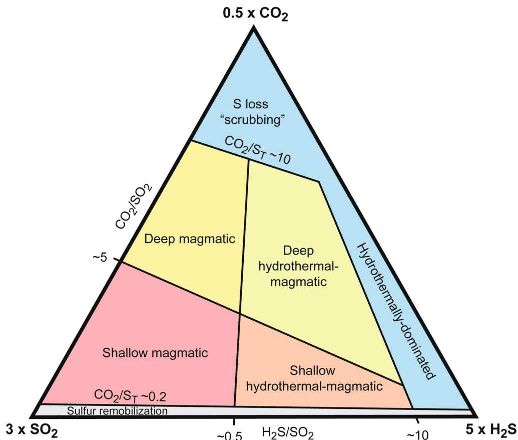
Fig. 6 Monitoring of gas compositions can provide crucial insight into the influence of the magmatic system. Generally, as a volcanic system reactivates, the gas emissions will evolve from \text{CO}_2 -rich to \text{SO}_2 -rich. This plot shows proposed generalized fields for the characterization of hydrothermal-magmatic gas emissions, based on recent studies of Central American volcanoes (Aiuppa et al. 2014; de Moor et al. 2016a, b, 2017a). The exact boundary lines would vary with tectonic setting and other factors (Aiuppa et al. 2017), but are shown here with key gas ratio values considered appropriate for Central American volcanoes
