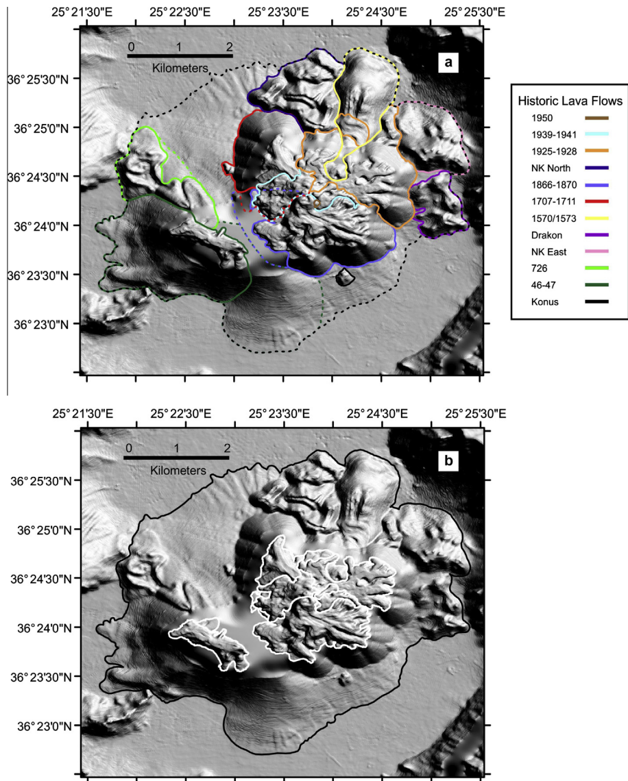
Fig. 3. Lava flow outlines for historic lava flows in the vicinity of the Kamenei islands. (a) New onshore/offshore lava flow outlines, mapped as part of this study. For the 46–47, 726, 1707–1711 and 1866–1870 flows the solid lines represent the minimum extent of the flows and the dashed line the possible maximum extent. The maximum extent of submarine talus deposits is shown by the black dashed line. (b) Onshore lava flows mapped by Pyle and Elliott [31] (white contours). The black contour represents the maximum extent of submarine talus deposits mapped during the current study.
