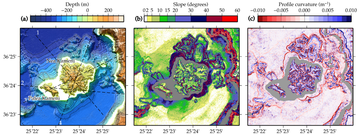
Fig. 2. Attribute maps of the Kamenei islands: (a) detailed topographic map (onshore & offshore data), (b) slope distribution map, (c) profile curvature map. The white and grey areas indicate no swath data. Black dashed lines mark the cross-sections shown in Fig. 4.
