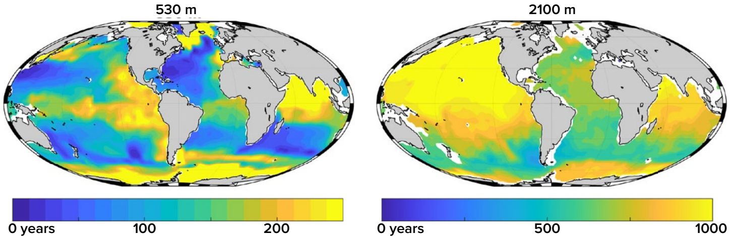
Figure 5. Durability of C sequestration as illustrated for two injection depths calculated for purposeful enhancements of the biological pump. Colors are median sequestration times from Siegel et al., 2021.
