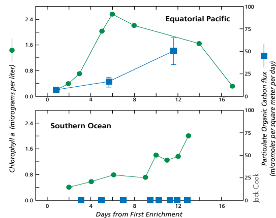
Chlorophyll (green) and carbon flux (blue) response to iron fertilization in the Equatorial Pacific and Southern Ocean.
