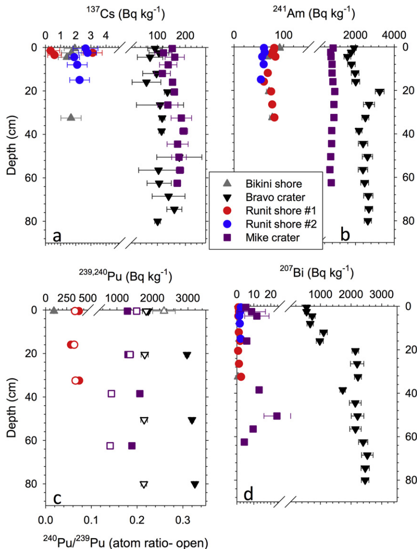
Fig. 5. Sediment core profiles vs. depth (cm-Y axis) for ^{137}\text{Cs} (a), ^{241}\text{Am} (b), ^{239,240}\text{Pu} (c) and ^{207}\text{Bi} (d). For each radionuclide the activities are along the upper x-axis in units of \text{Bq kg}^{-1} dry weight. For Pu, also shown are the ^{240}\text{Pu}/^{239}\text{Pu} atom ratios as open symbols with scale along the lower x-axis. Sample key is shown for Bikini shore (gray triangles), Bravo Crater (black inverted triangles), Runit shore (#1 and #2 are two sites, red and blue circles, respectively) and the Mike Crater (purple square). Error bars are shown if larger than the symbol size for each measurement. Data are in Table S2.
